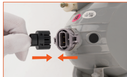
Fig.5: Attach the LED bulb connector with the original vehicle connector and reinstall the rubber cover(if present).
